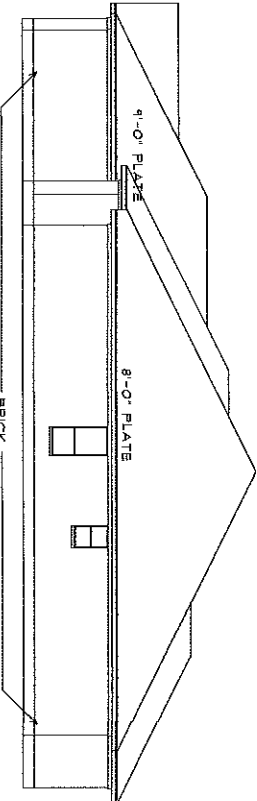
RIGHT ELEVATION 1/8"
